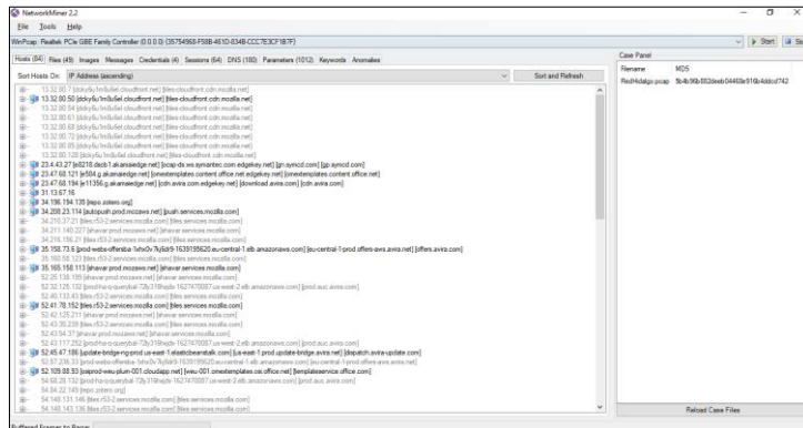
Fig. 3.16. Herramienta NetworkMiner.
