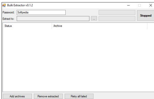
Fig. 2.14. Bulk Extractor.
